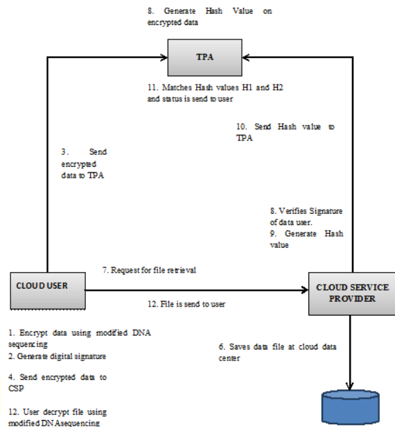
Fig.1. Proposed File Storage Methodology
