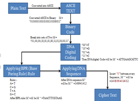
Fig.2. DNA Encoding Process
