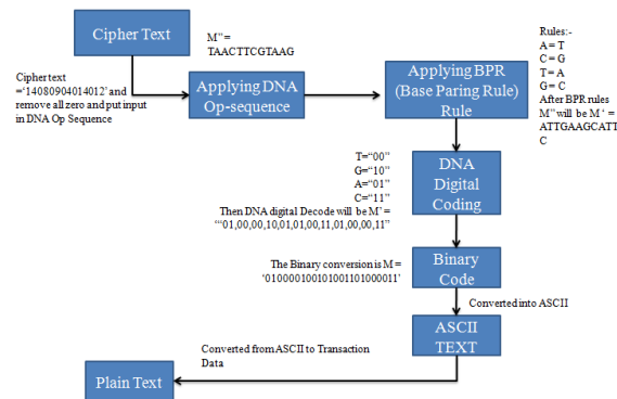
Fig.3. DNA Decoding Process
