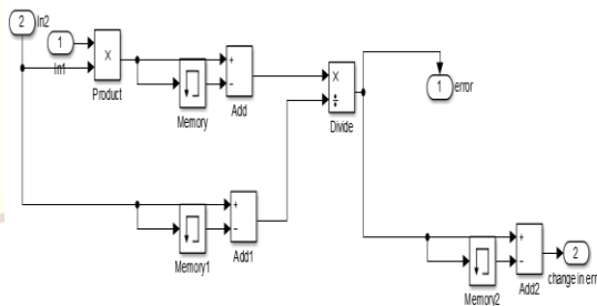
Figure 3: Subsystem for Power Error and Change in Error
