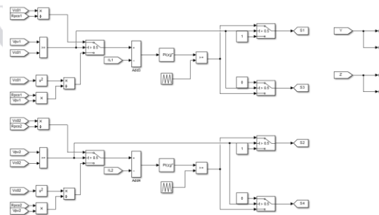
Figure 2: ANFIS Controller for Two PV inverter
