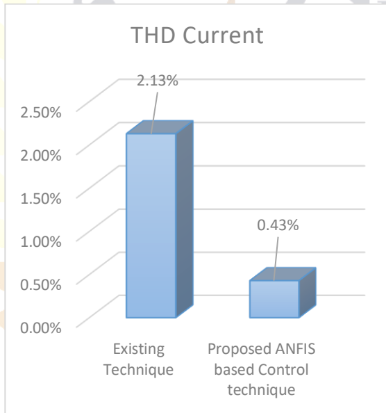
Figure 8: THD comparison for current
