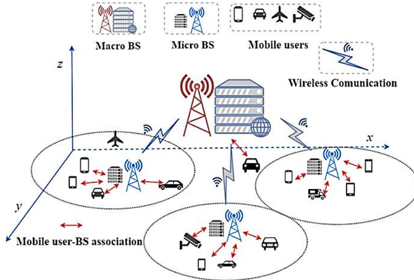
Figure 1: System Model
