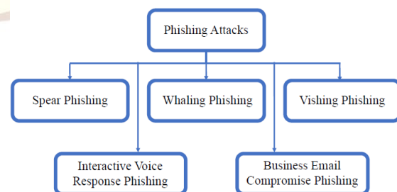
Figure 5. Phishing attacks.
