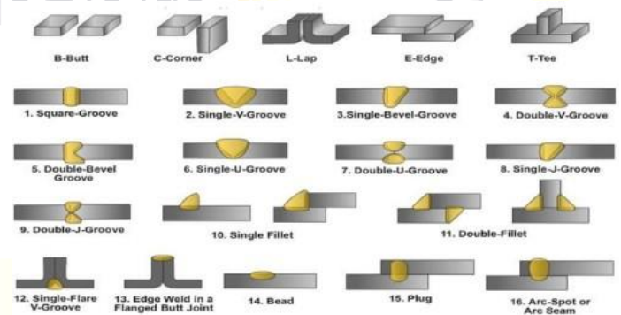
Figure.1.2: Types of welding joints [2]
