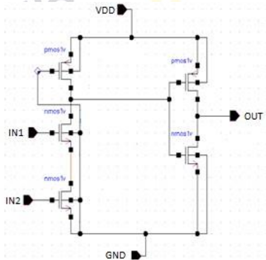
Fig. 2 Schematic of two input AND Gate Using Pseudo NMOS Logic
