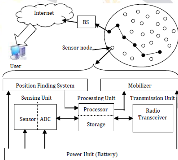
Figure 1: System Model of Wireless Sensor Network [4]
